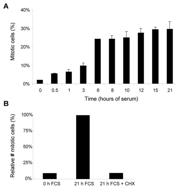
Figure 1 Evidence for a G_2 restriction point. A. Cell cycle re-entry from G_2 requires 6 hours of mitogen-stimulation. Serum-starved cells were stimulated by the addition of serum-containing medium. Subsequently, at the indicated times medium was replaced with serum-free medium containing Taxol for the last 9 hours. At 21 hours cells were harvested and fixed in 70% ethanol and mitotic entry was determined by MPM2 FACS staining. Error bars indicate the standard deviation for two experiments. B. Cell cycle re-entry from G_2 requires protein synthesis. Serum-starved cells were serum-stimulated in the absence or presence of 50 \mu g/ml cycloheximide (CHX). Cells were fixed at 21 hours and mitotic entry was determined by MPM2 FACS staining. The level of MPM2 positivity in serum-stimulated cells at 21 hours is set at 100%.
