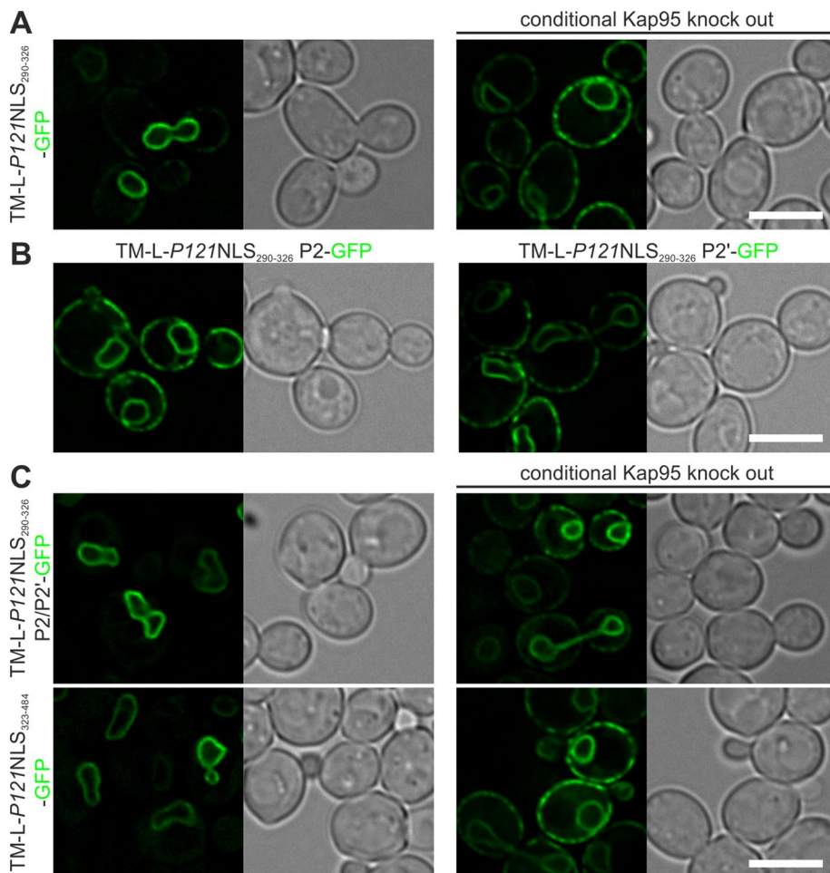
FIGURE 3: The IBB-like region is sufficient for INM targeting, and the Pom121 NLS region consists of redundant NLSs. (A) The IBB-like region of Pom121 NLS alone in TM-L-P121NLS 290-326 -GFP is sufficient to induce Kap95-dependent INM accumulation of the reporter protein, and (B) substitution of the lysine residues at the P2 or P2' positions by alanine residues is sufficient to abolish NE accumulation. (C) Lysine-to-alanine mutation at the P2 and P2' positions of the IBB-like region of the NLS of Pom121 in the context of the full Pom121 NLS cluster (TM-L-P121NLS 290-484 P2/P2'-GFP) or removal of the IBB-like region from the full Pom121 NLS (TM-L-P121NLS 323-484 -GFP) did not alter Kap95-dependent INM accumulation of the indicated reporter proteins. Scale bars, 5 μm.
