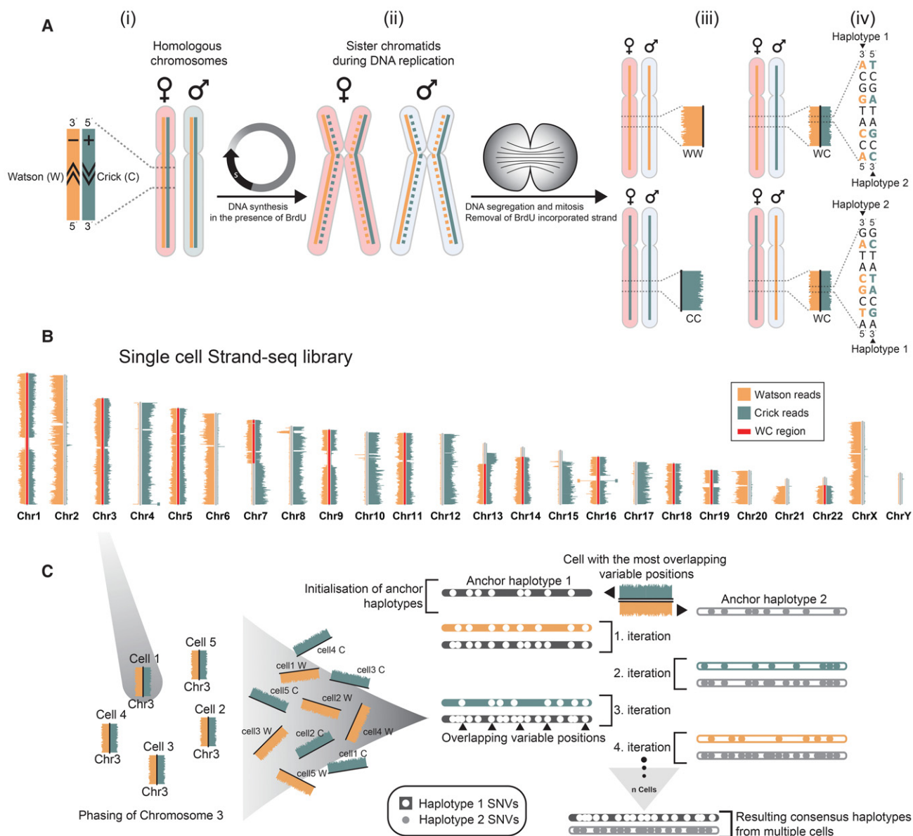
Figure 1. Direct whole-chromosome haplotyping using single-cell template strand sequencing (Strand-seq). (A,i) Two homologous chromosomes, one originating from the mother (light red) and one from the father (light blue), are shown. Each homolog is composed of a positive template strand (Crick; teal) and a negative template strand (Watson; orange). (ii) Cells incorporate BrdU during DNA replication, generating hemi-substituted sister chromatids containing one BrdU-negative template strand (solid line) and one BrdU-positive newly synthesized strand (dashed line). (iii) Segregation of sister chromatids in two daughter cells follows the depicted combinations of maternal and paternal template strands. The newly formed DNA strands containing BrdU are selectively removed in daughter cells during library preparation, such that only the original template DNA strands are sequenced. Read density along a chromosome is plotted as horizontal bars. (iv) When daughter cells inherit one Crick and one Watson template strand for a particular chromosome, we can use strand directionality to directly assign all reads to separate haplotypes. (B) Example of a single-cell Strand-seq library, generated from HapMap cell line NA12878. Each chromosome is represented as a vertical ideogram, and the distribution of directional sequencing reads is represented as horizontal lines along each chromosome, with Watson in orange and Crick in teal. WC regions that were selected for haplotype phasing are highlighted by red bars. (C) The custom phasing algorithm StrandPhase processes one chromosome at a time. Cells that inherit one Crick and one Watson template strand for a particular chromosome are selected as input, and the SNVs identified on each template strand are used to derive each single-cell haplotype. In the first iteration, anchor haplotypes are established by pairing single-cell haplotypes exhibiting the highest number of overlapping heterozygous SNVs. This is used to initialize the consensus haplotypes “H1” and “H2,” which are further built upon in subsequent iterations. In the second iteration, the second most-dense single-cell haplotype is considered and compared to both consensus haplotypes, and any new SNVs are added to the consensus haplotype showing the best concordance. With each iteration, the consensus haplotypes are extended until no additional single-cell haplotype can be reliably assigned to the one of the consensus haplotypes.
